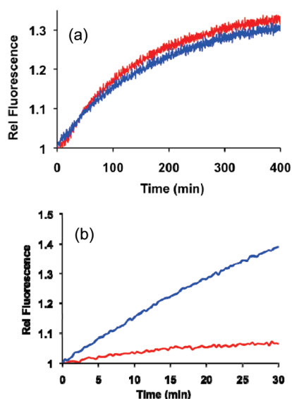
Figure 4. (a) Phosphorylation of the Abl sensor 11 ( \lambda_{\text{ex}} = 400 nm, \lambda_{\text{em}} = 525 nm) by MYL (red) and MYL-R (blue) lysates. (b) Phosphorylation of the Lyn sensor 9 ( \lambda_{\text{ex}} = 665 nm, \lambda_{\text{em}} = 705 nm) by MYL lysates (red) and MYL-R lysates (blue). Lysates contain all endogenous protein kinases and were normalized for total protein content as described in Methods (Protein Kinase Assays). Abl and Lyn kinase activities were monitored simultaneously during the course of the experiments.
