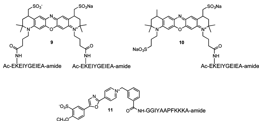
Figure 2. Structures of the Lyn ( 9 and 10 ) and Abl ( 11 ) substrates.
