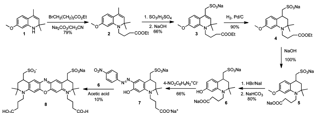
Figure 1. Synthesis of the oxazine diacid 8 . The latter was coupled to the Lys side chain of the Lyn peptide substrate Ac-Glu- Lys -Glu-Ile-Tyr-Gly-Glu-Ile-Glu-Ala-amide, to furnish the 2:1 peptide–oxazine conjugate 9 .
