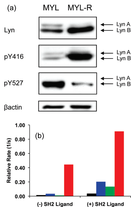
Figure 6. (a) Total Lyn A and B, pY416, and pY527 content in MYL and MYL-R cell lines. (b) Initial phosphorylation rate of Lyn sensor 9 with Lyn-precleared MYL lysates (black), MYL lysates (blue), Lyn-precleared MYL-R lysates (green), and MYL-R lysates (red).
