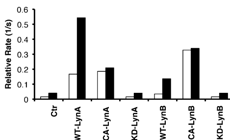
Figure 5. Initial rate of the phosphorylation of Lyn sensor 9 [without (unfilled) and with (filled) SH2 ligand (200 \mu M Ac-pTyr-Glu-Glu-Ile-Glu)] by HEK293 cells transfected with the indicated constructs (where Ctl = control-transfected HEK293 cells). Lysates contain were normalized for total protein content as described in Methods (Protein Kinase Assays).
