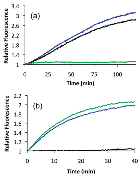
Figure 3. (a) Phosphorylation of 9 ( \lambda_{\text{ex}} = 665 \text{ nm} , \lambda_{\text{em}} = 705 \text{ nm} ) by purified Lyn B (black), Lyn B/Abl (blue), and Abl (green). (b) Phosphorylation of 11 ( \lambda_{\text{ex}} = 400 \text{ nm} , \lambda_{\text{em}} = 525 \text{ nm} ) by purified Lyn B (black), Lyn B/Abl (blue), and Abl (green).
